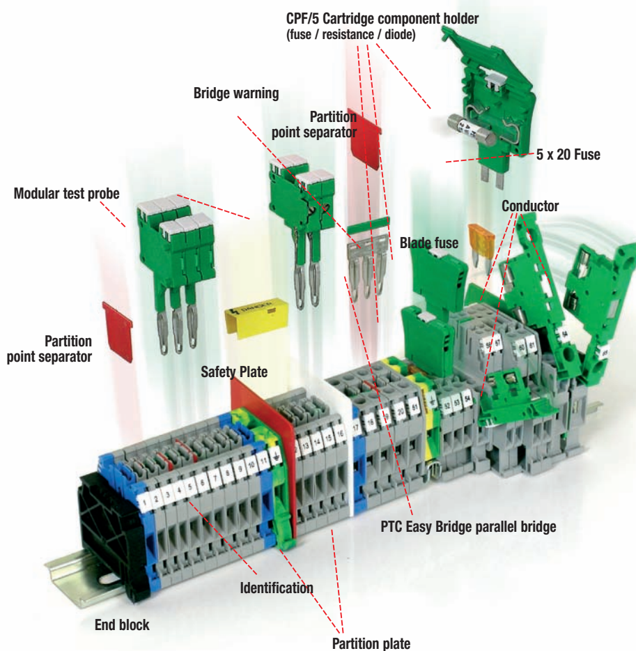
CBC series terminal block and relative accessories.
